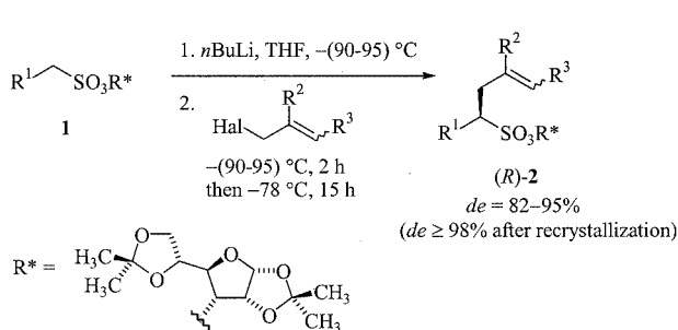
Scheme 1. Asymmetric \alpha -allylation of chiral sulfonates 1 to afford the product ( R )- 2
