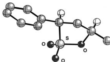
Figure 2. X-ray crystal structure of 5c
