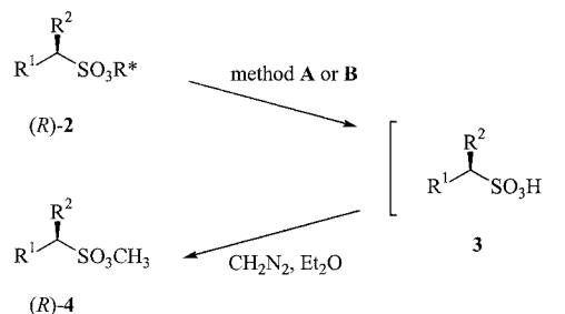
Scheme 2. Removal of the chiral auxiliary to form the methyl sulfonates ( R )- 4 : Method A: Pd(OAc) 2 , EtOH/H 2 O, reflux, 4 days. Method B: 2% TFA/EtOH, reflux, 24 h
