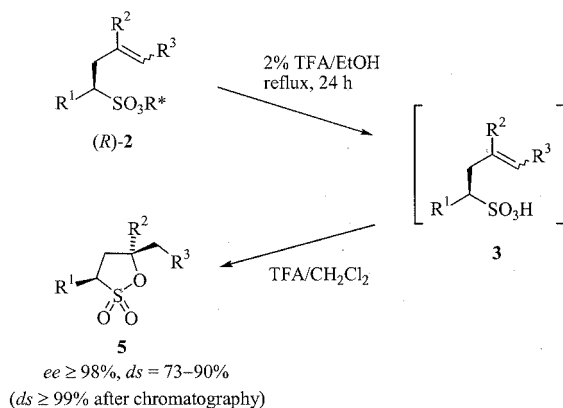
Scheme 3. Removal of chiral auxiliary and cyclization of the sulfonic acid 3 to afford the \gamma -sultones 5
