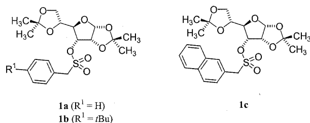
Figure 1. The enantiopure sulfonates 1a–c
