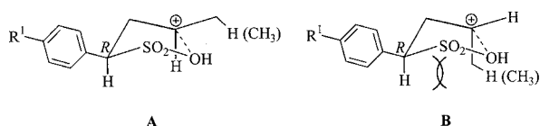
Figure 3. Proposed transition state of the cyclization of sulfonic acids
